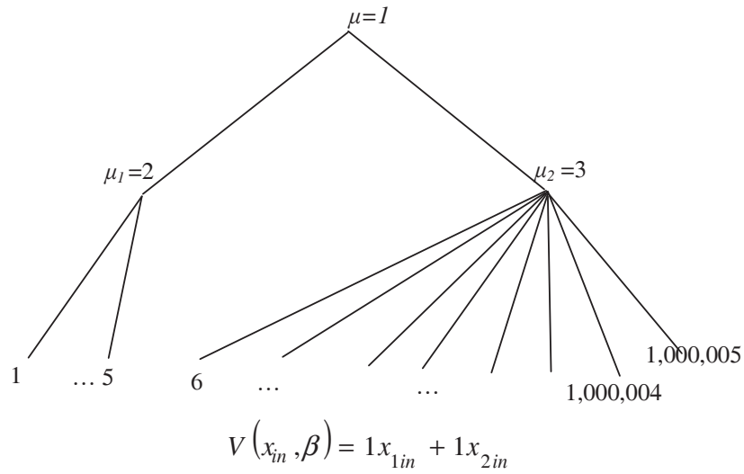
Figure 3 Monte Carlo Experiment: Nesting Structure. 1,00,005 Alternatives
