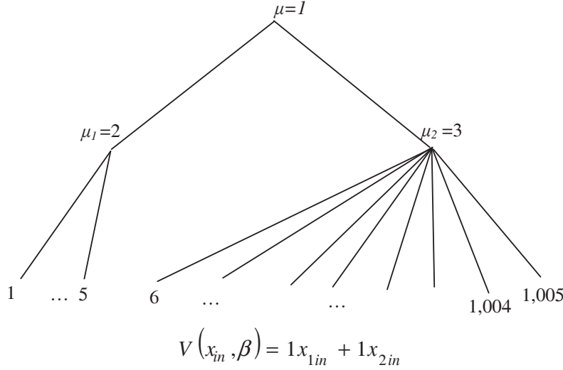
Figure 1 Monte Carlo Experiment: Nesting Structure. 1,005 Alternatives
